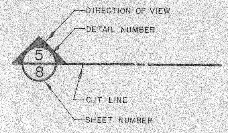
REFERENCE BUBBLE DETAIL
